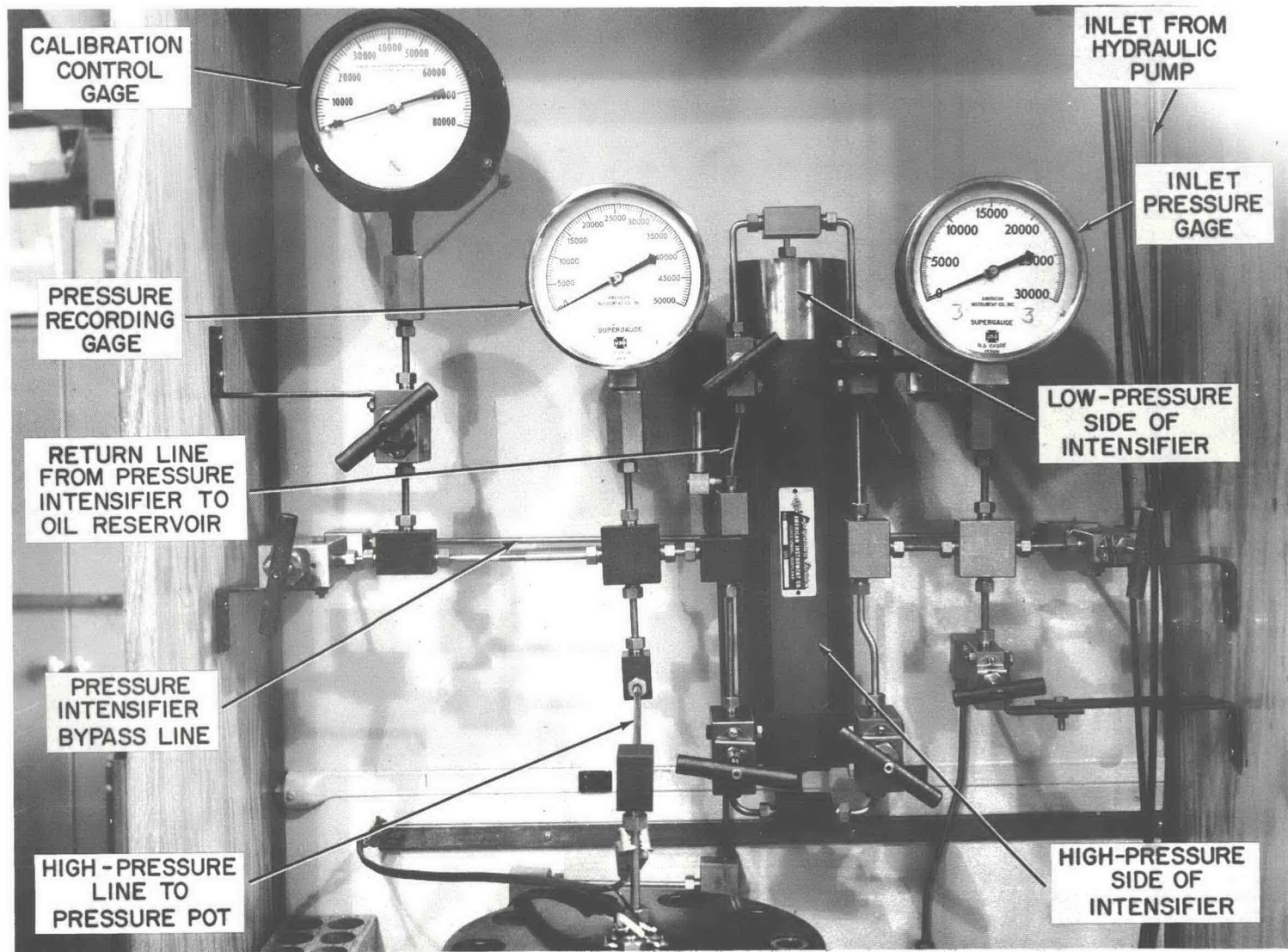
FIG. 11 HIGH-PRESSURE CONTROL SYSTEM
